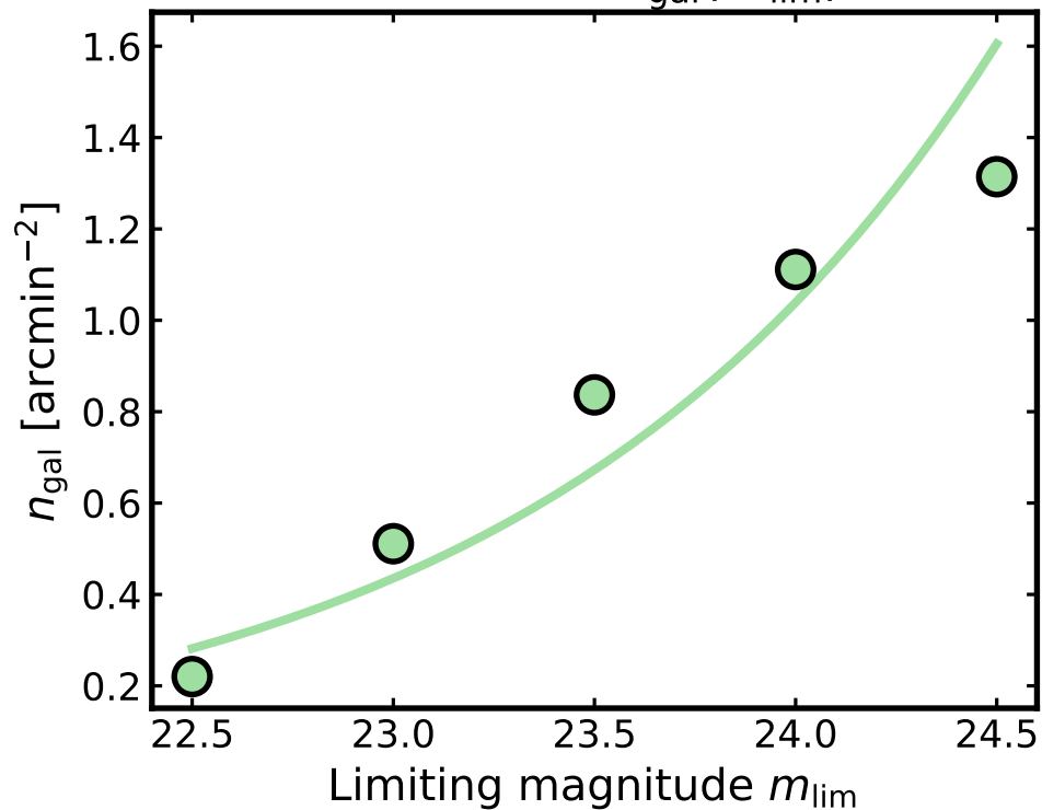
Calibrated n_{\text{gal}}(m_{\text{lim}})
