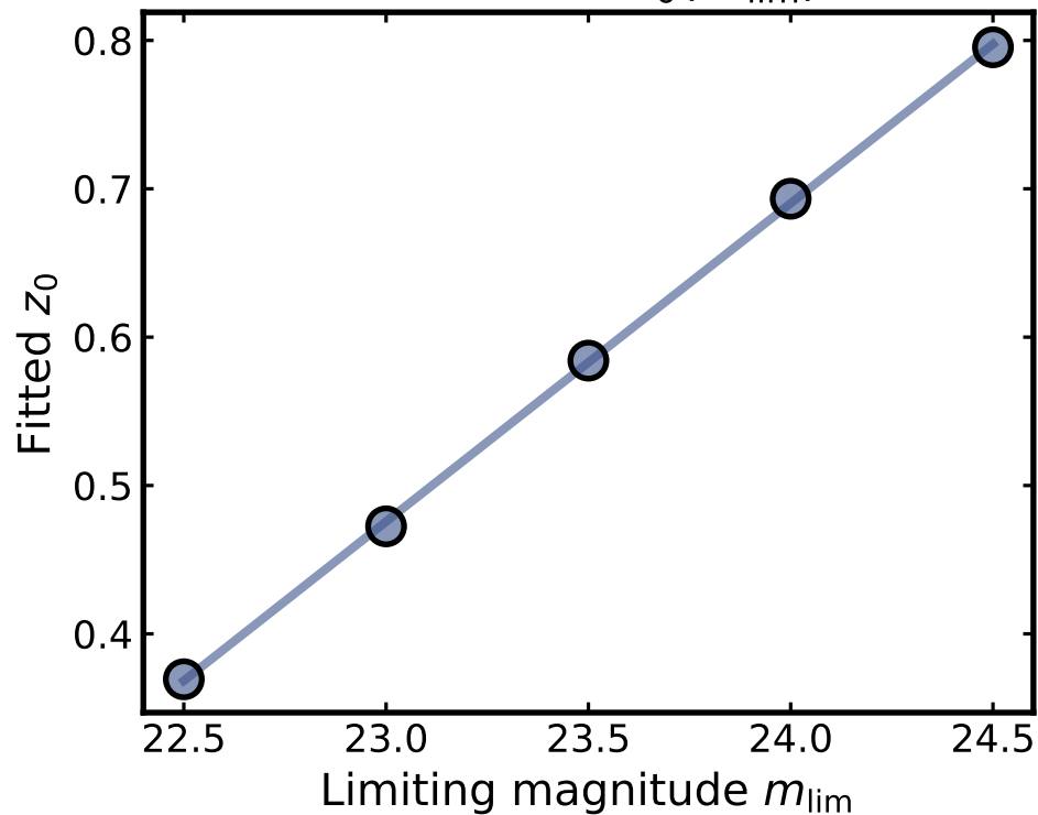
Calibrated z_0(m_{\text{lim}})
