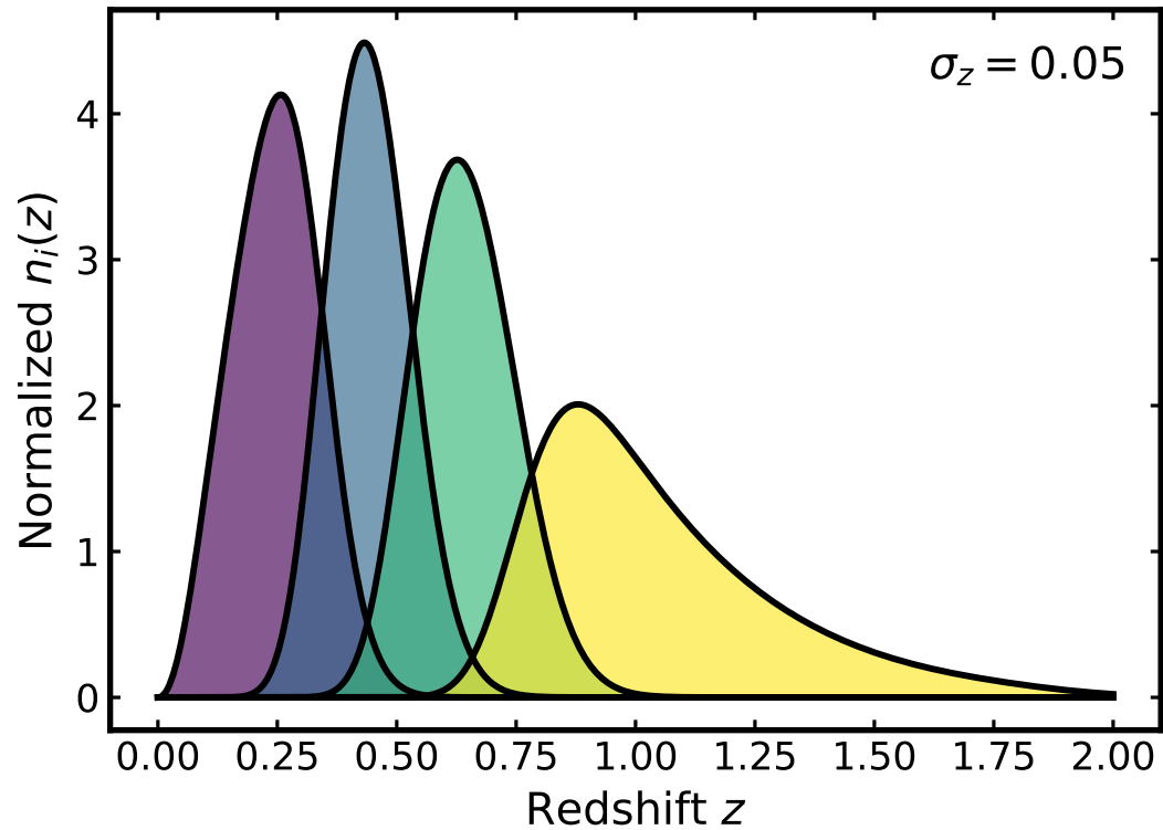
Shared scatter
