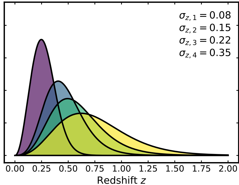
Per-bin scatter
