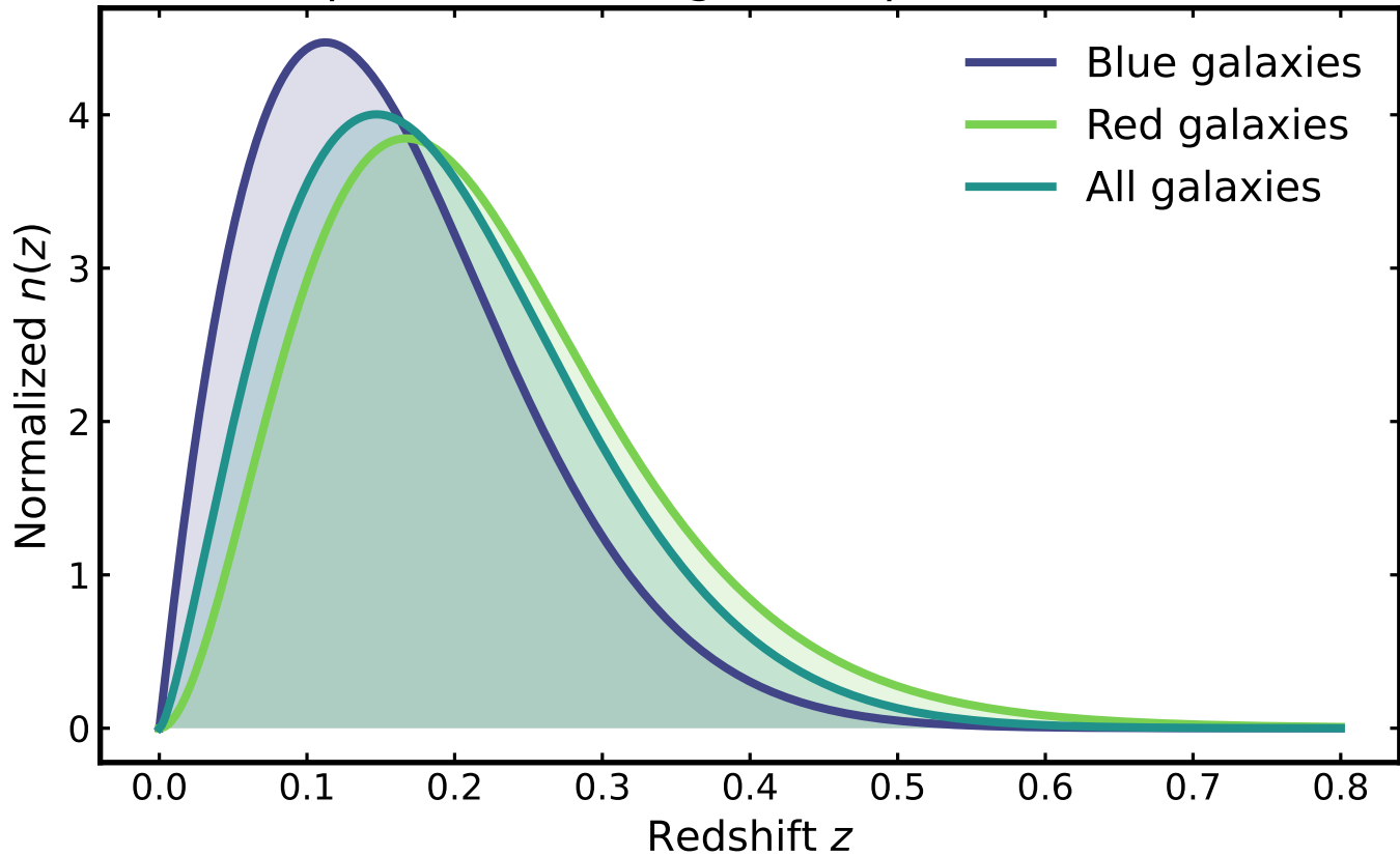
Blue and red split LF modelling of the parent redshift distribut
