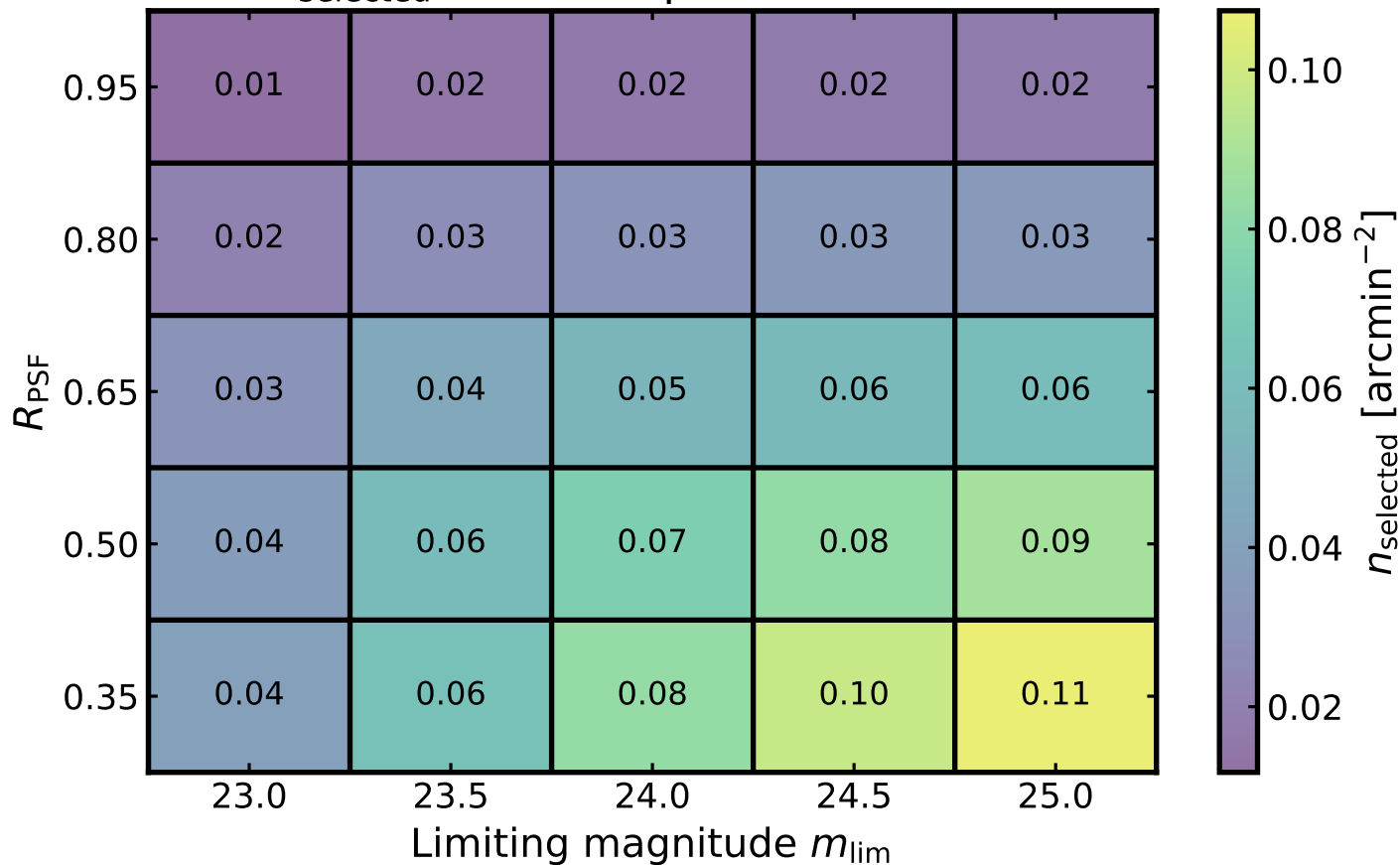
n_{\text{selected}} across depth and PSF size
