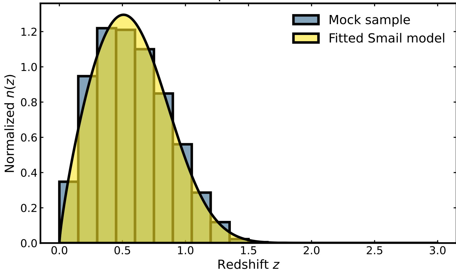
Mock redshift sample and calibrated Smail fit
