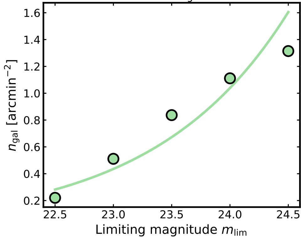
Calibrated n_{\text{gal}}(m_{\text{lim}})
