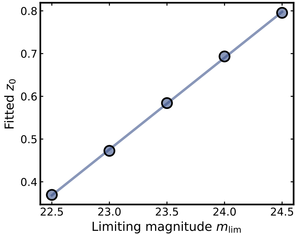
Calibrated z_0(m_{\text{lim}})
