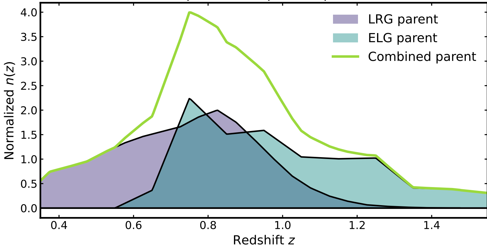
DESI parent sample composition
