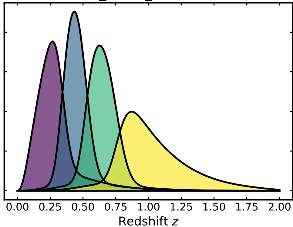
outlier_mean_offset = 0.12
