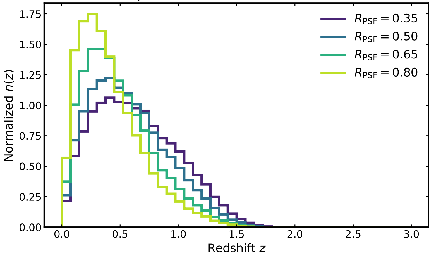
PSF-dependent source redshift distributions
