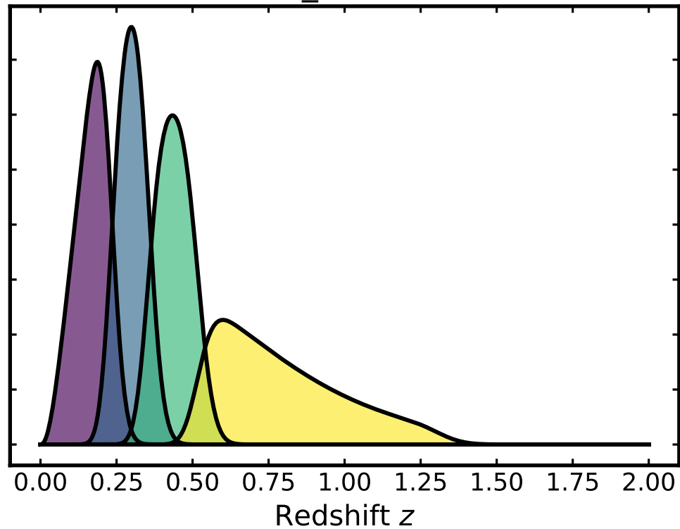
mean_scale=1.5
