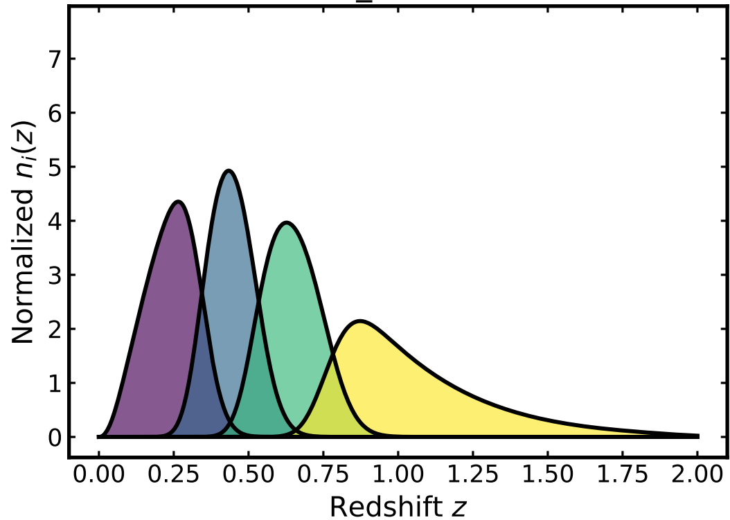
mean_scale=1.0
