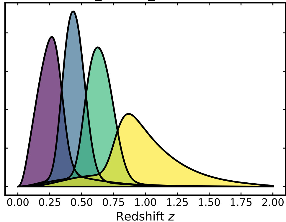
outlier_scatter_scale = 0.35
