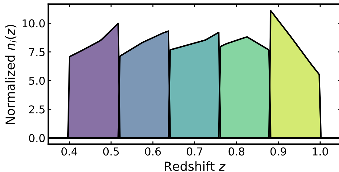
DESI LRG: five bins
