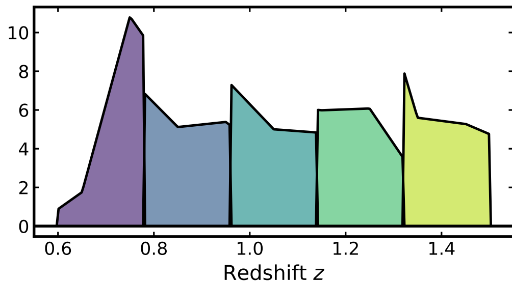
DESI ELG: five bins
