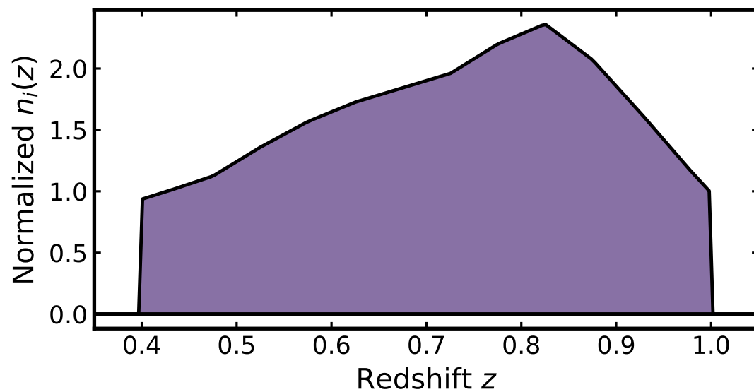
DESI LRG: one bin
