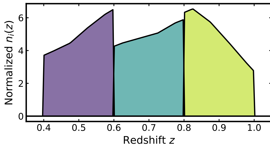
DESI LRG: three bins
