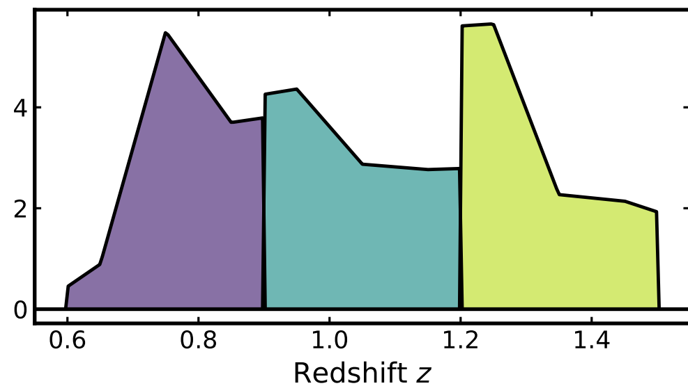
DESI ELG: three bins
