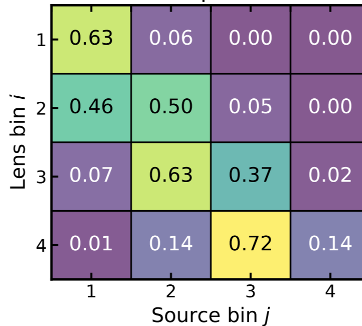
Overlap matrix
