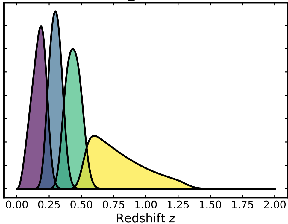
mean_scale=1.5
