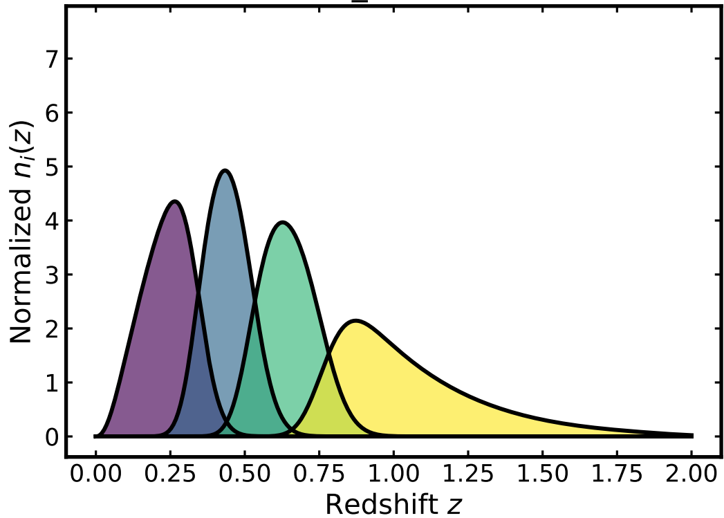
mean_scale=1.0
