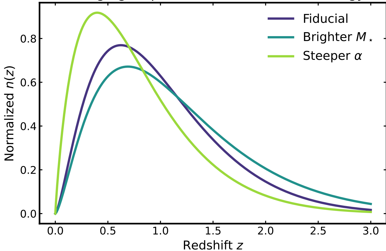
Changing LF parameters at fixed cosmology
