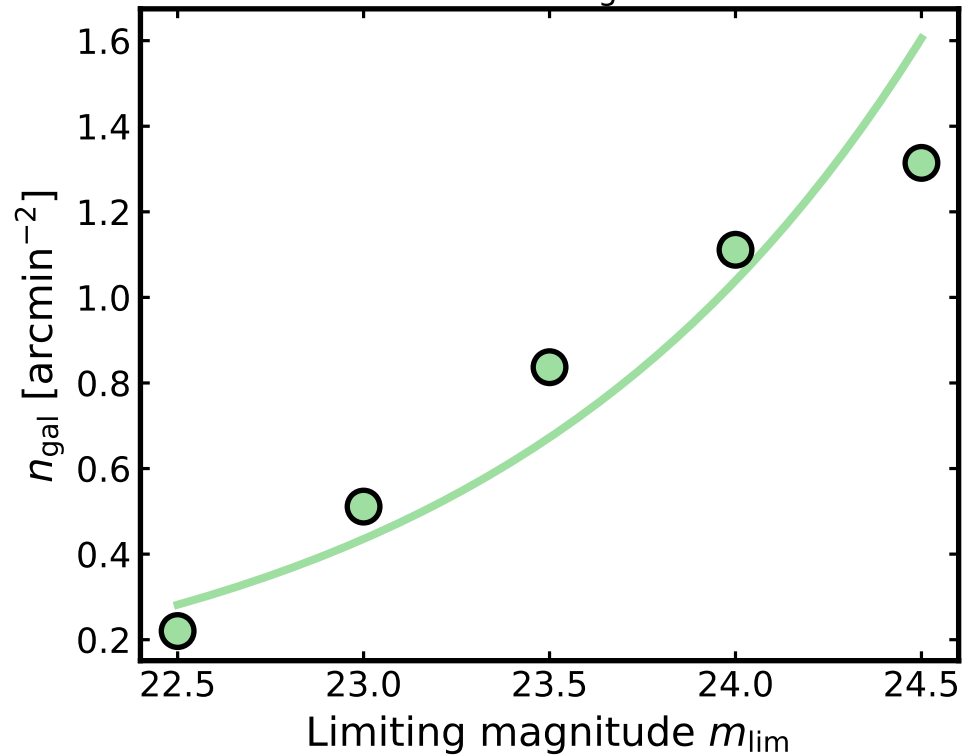
Calibrated n_{\text{gal}}(m_{\text{lim}})
