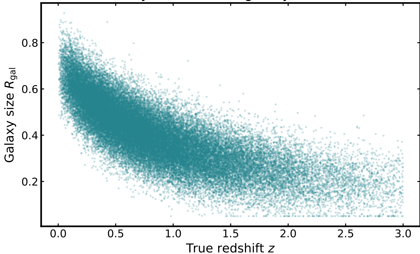
Synthetic mock galaxy sizes
