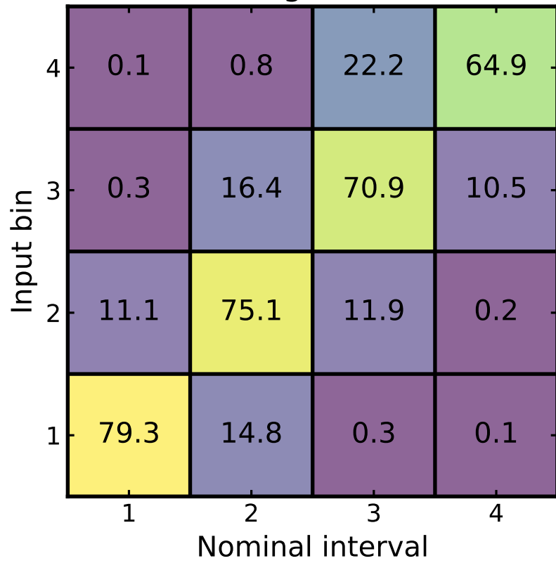
Leakage matrix
