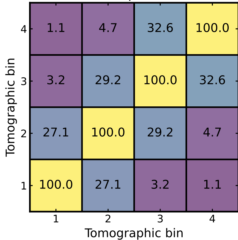
Overlap matrix
