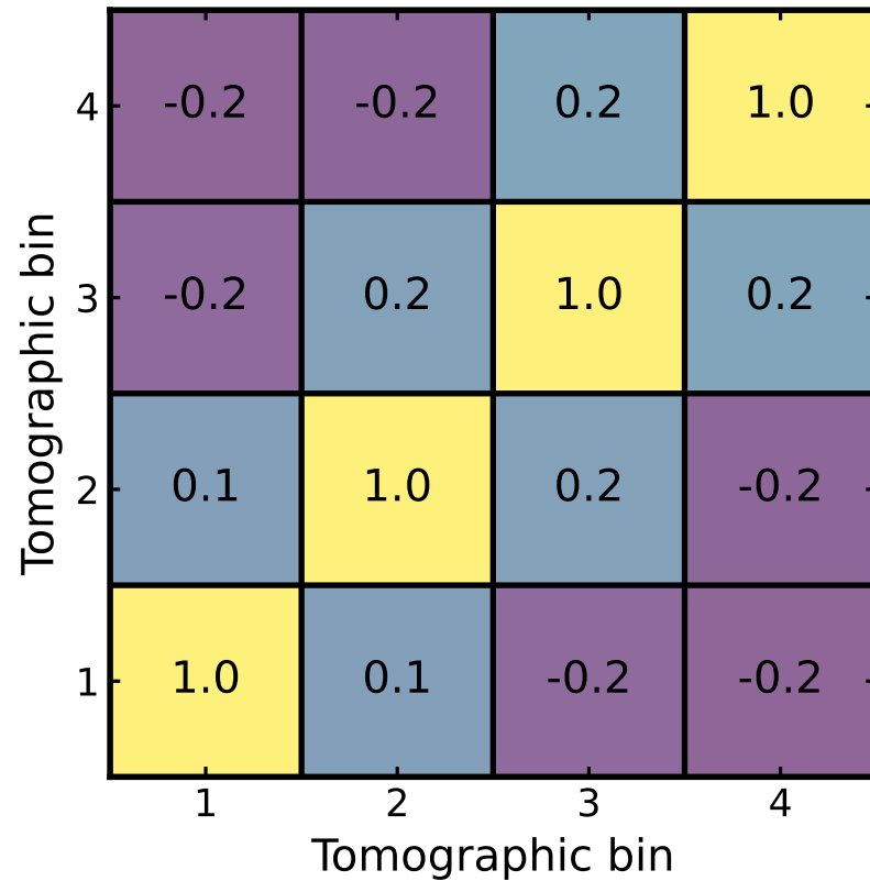
Pearson matrix
