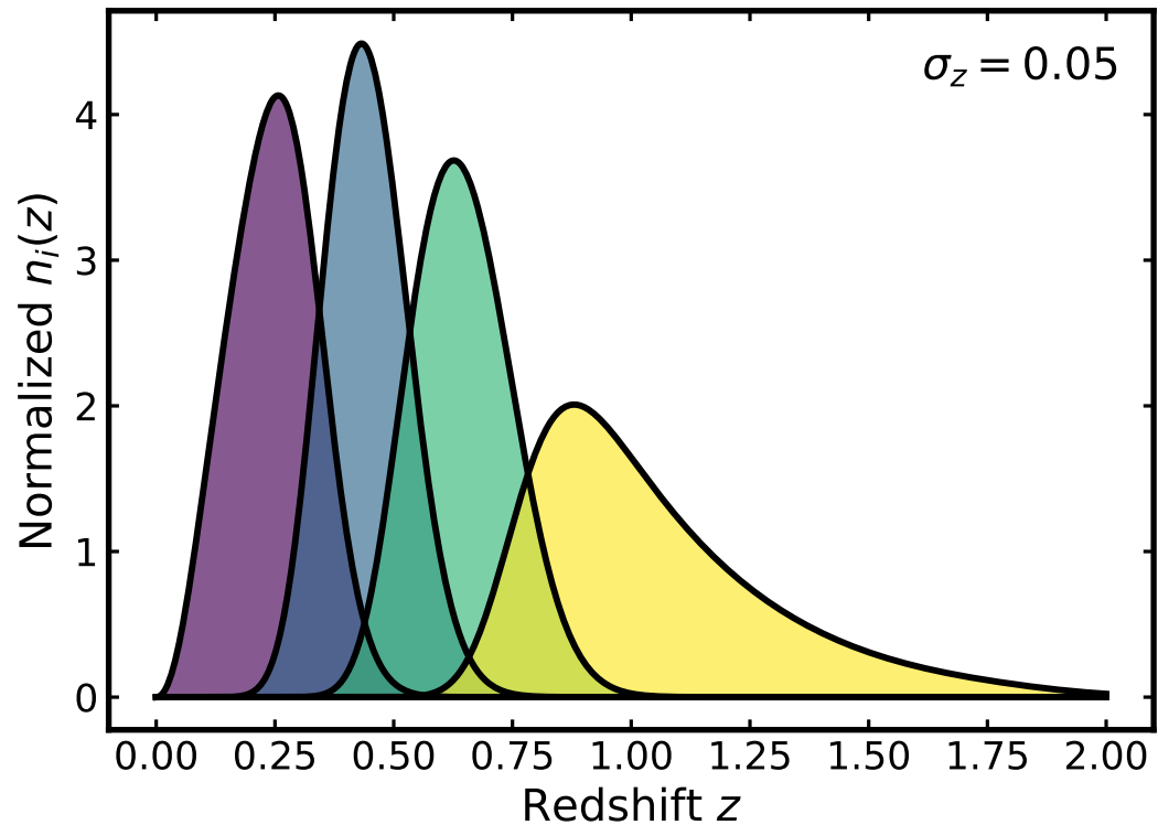
Shared scatter
