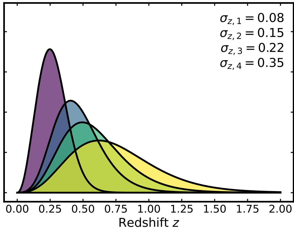
Per-bin scatter
