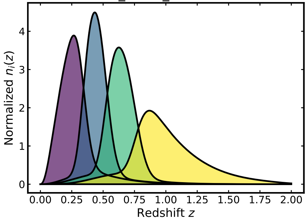
outlier_mean_offset = 0.02
