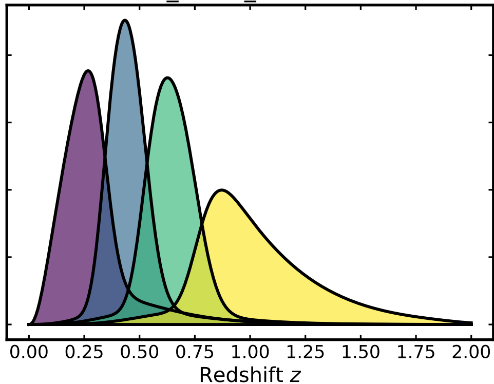
outlier_mean_offset = 0.12
