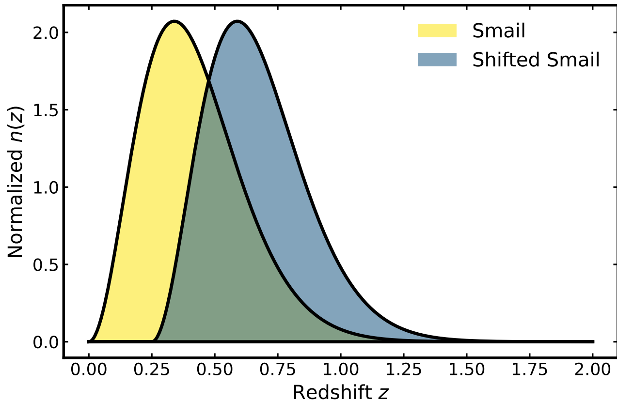
Standard vs shifted Smail distribution
