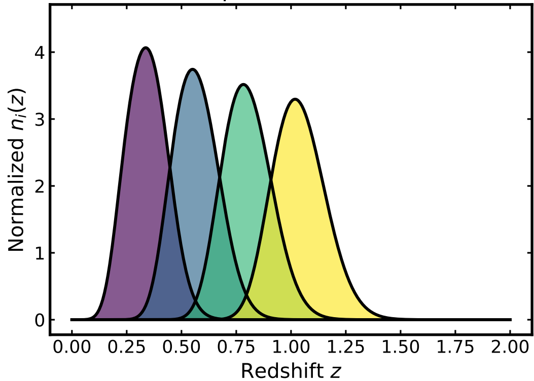
Equidistant bins
