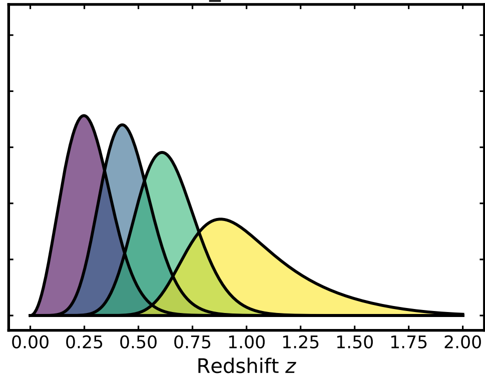
scatter_scale = 0.08
