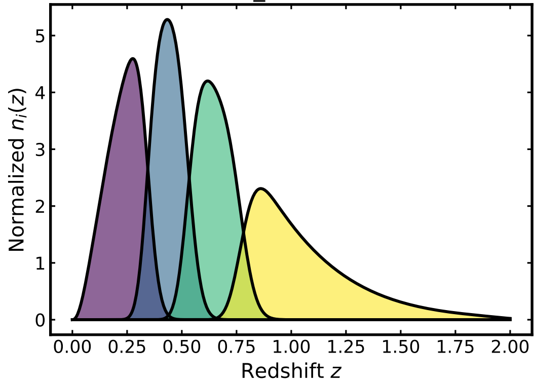
scatter_scale = 0.03
