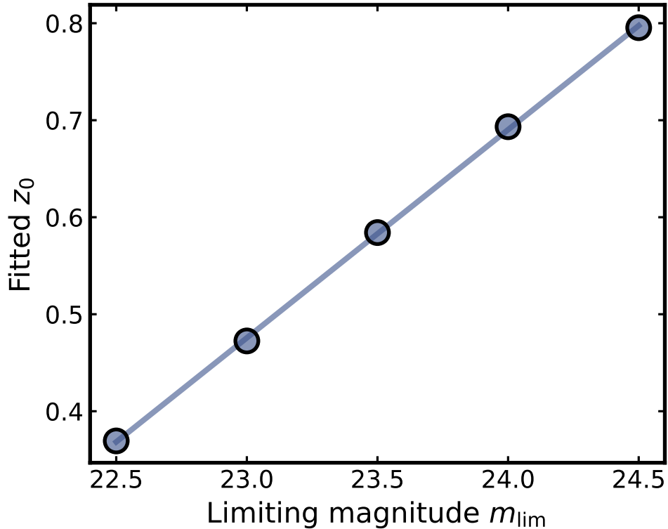
Calibrated z_0(m_{\text{lim}})
