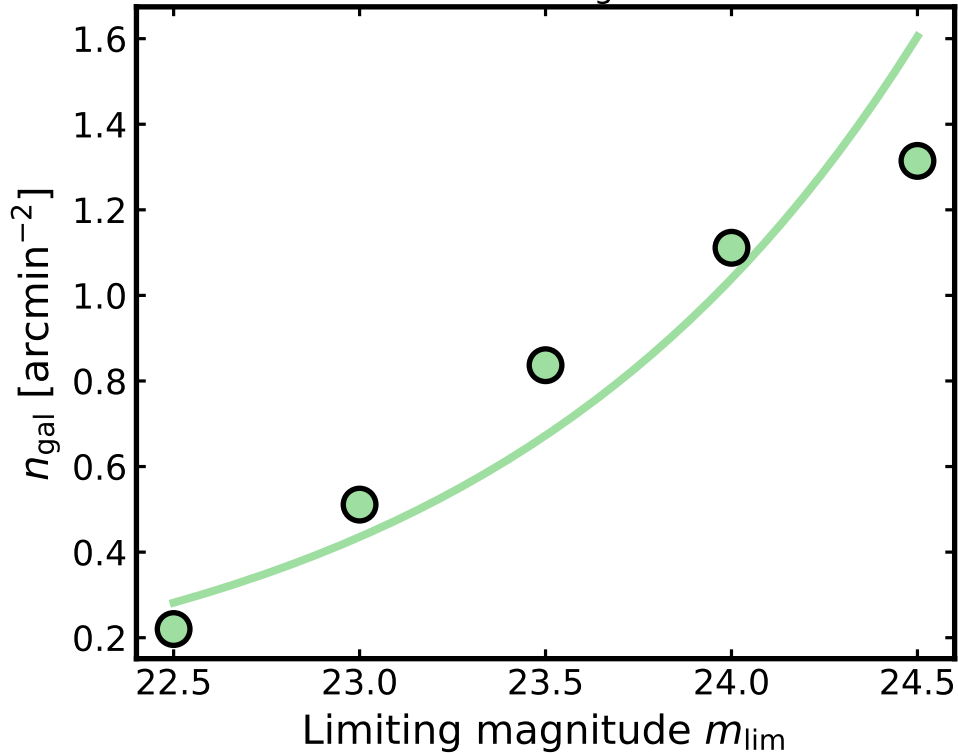
Calibrated n_{\text{gal}}(m_{\text{lim}})
