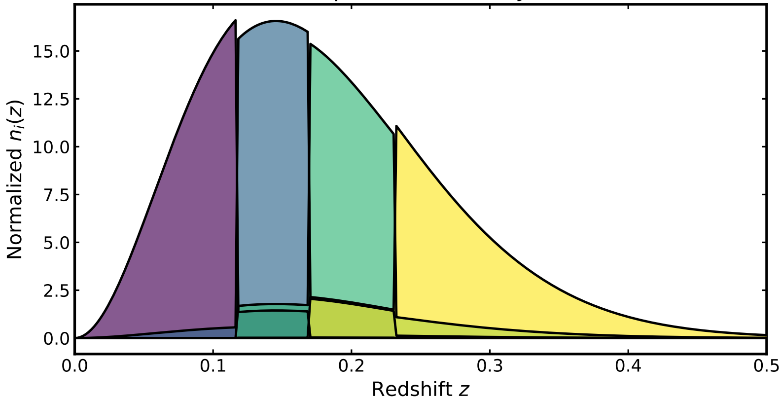
Unified spec-z uncertainty model
