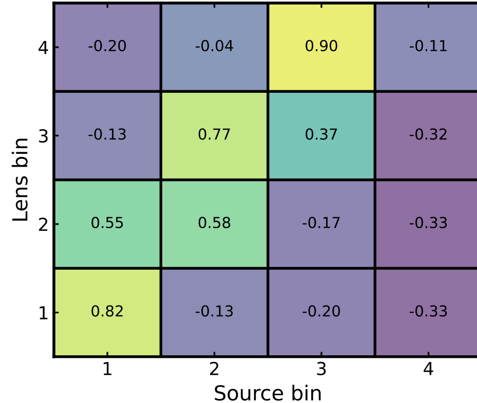
Between-sample Pearson
