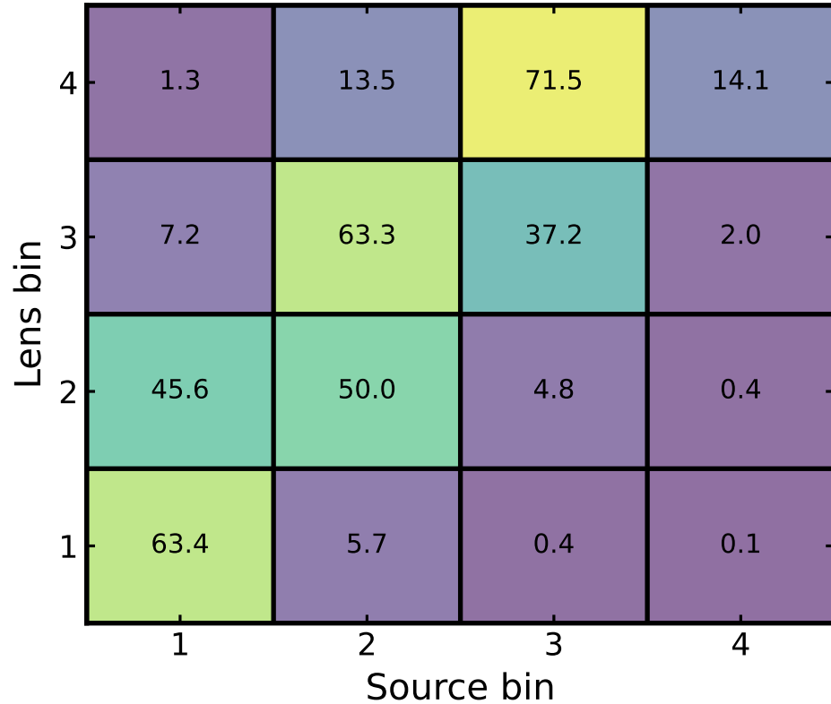
Between-sample overlap
