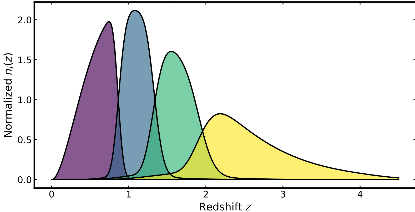
Unified photo-z uncertainty model
