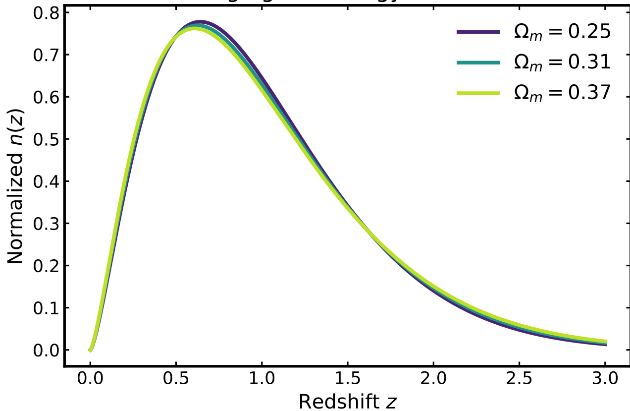
Changing cosmology at fixed LF
