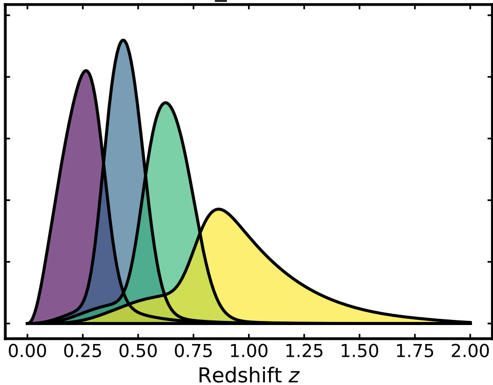
outlier_frac = 0.08
