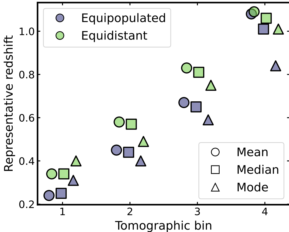
Peak-location summaries
