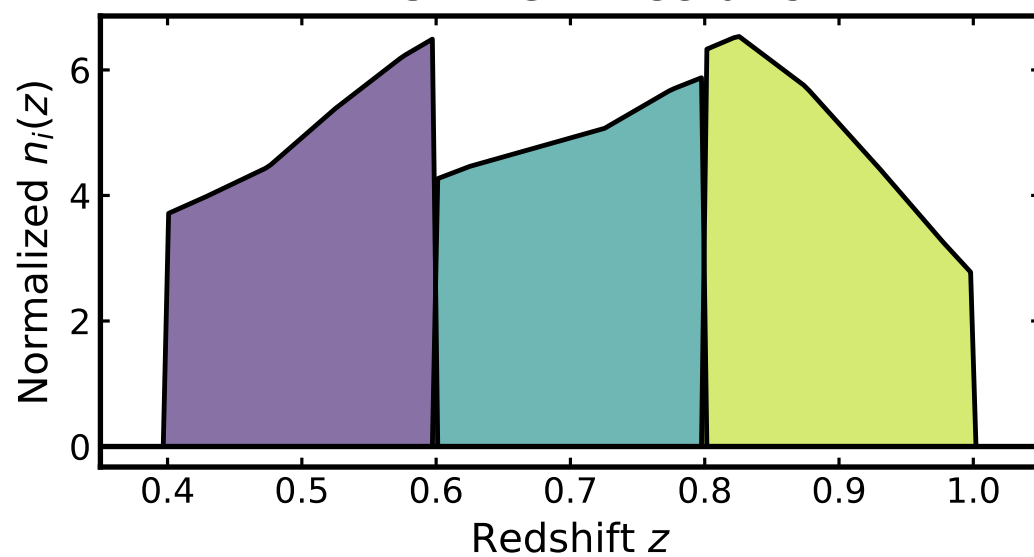
DESI LRG: three bins
