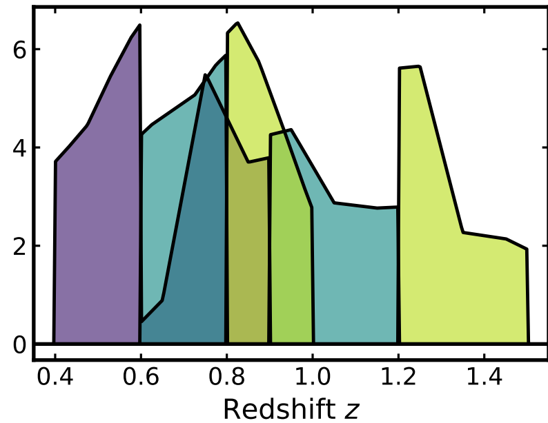
Combined LRG + ELG bins
