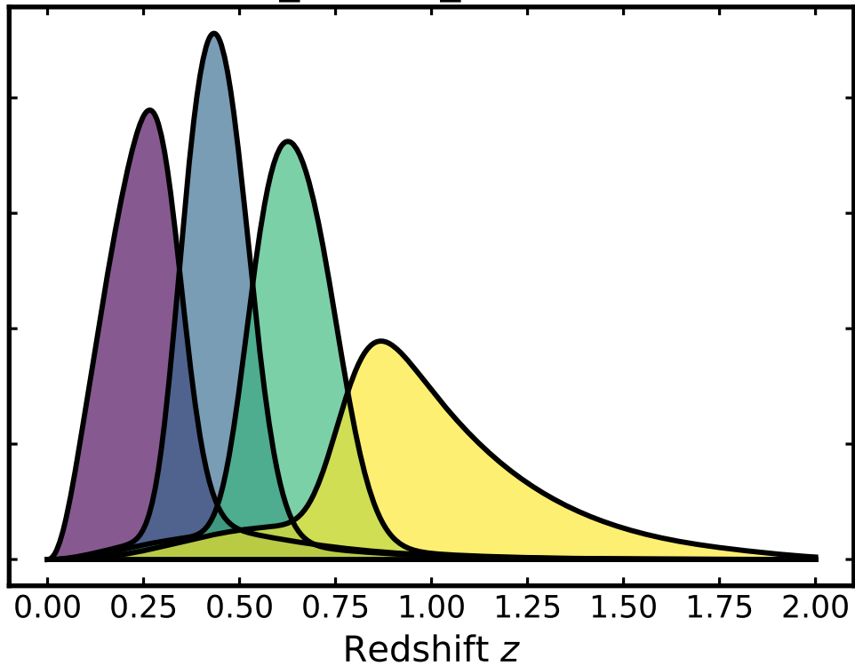
outlier_scatter_scale = 0.35
