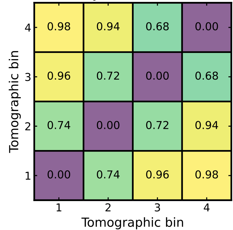
JS distance
