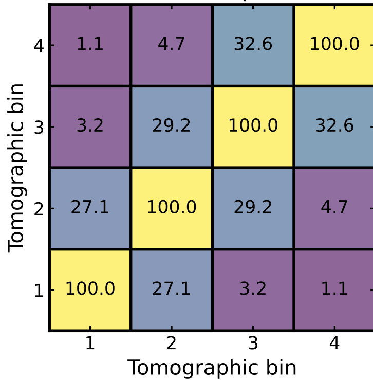
Min overlap [%]
