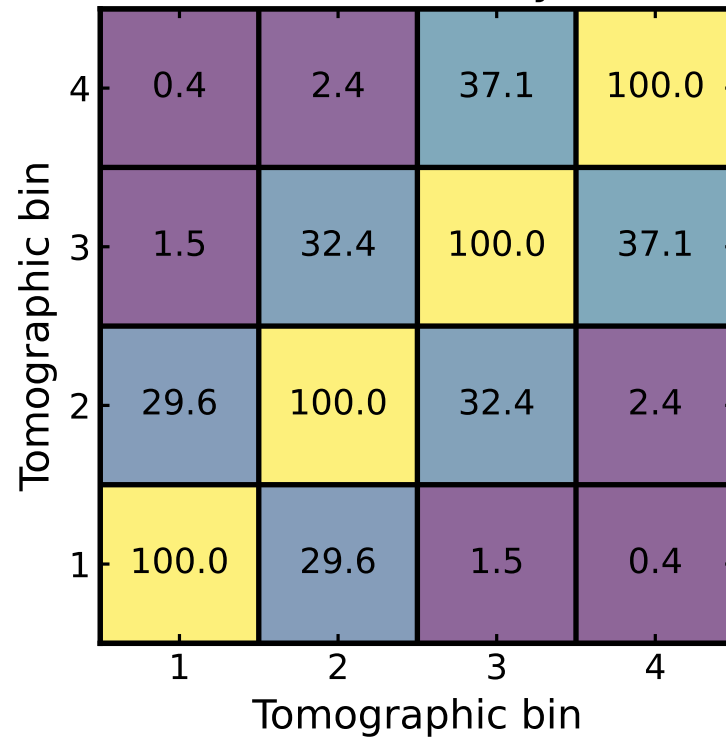
Cosine similarity [%]
