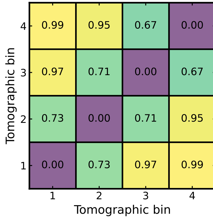
TV distance
