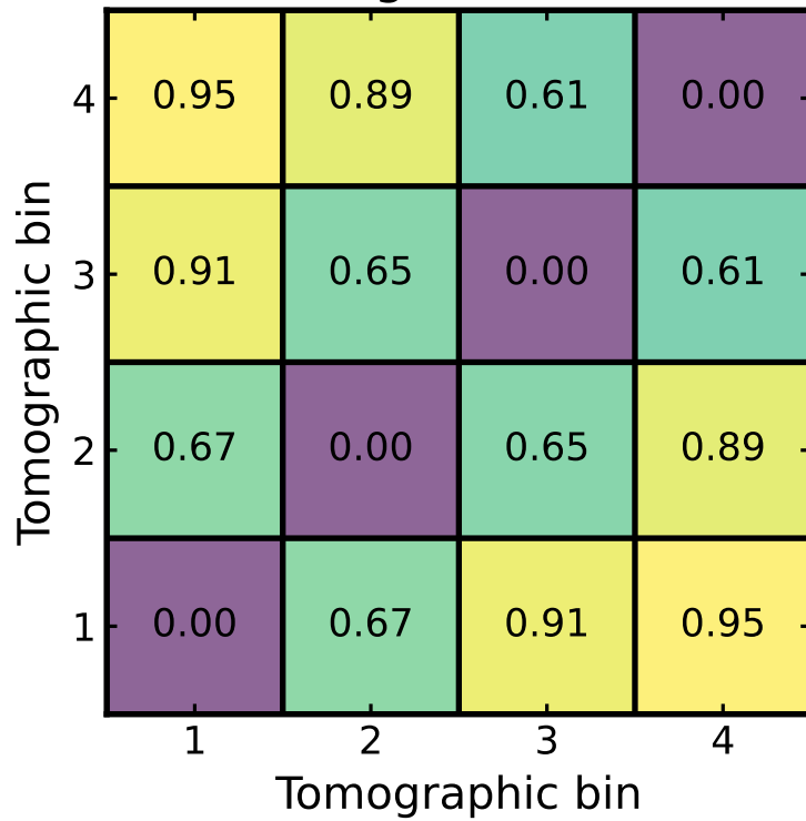
Hellinger distance
