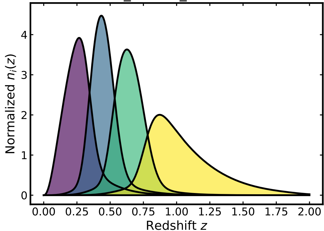
outlier_scatter_scale = 0.15
