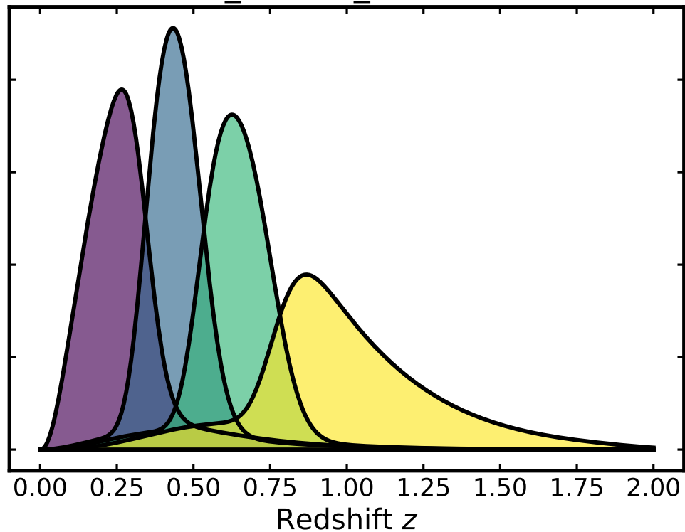
outlier_scatter_scale = 0.35
