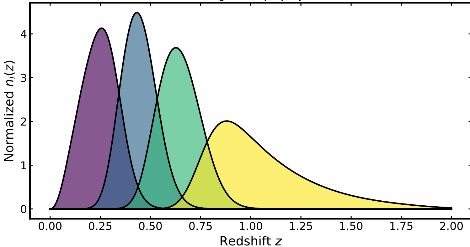
Photo-z binning: 4 equipopulated bins
