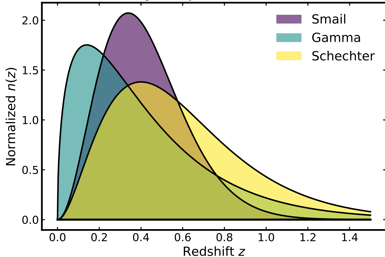
Survey-like parent n(z) models
