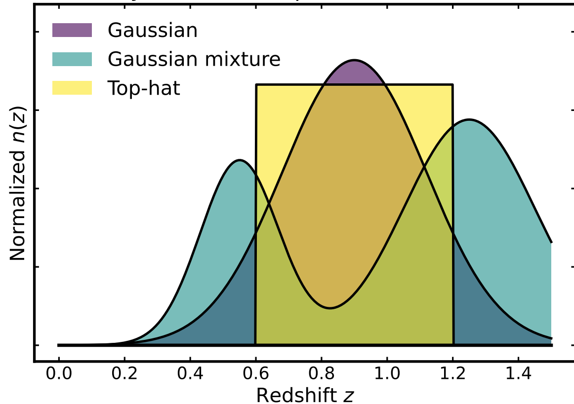
Toy and mixture parent n(z) models
