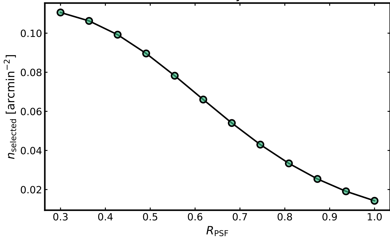
Selected source density versus PSF size
