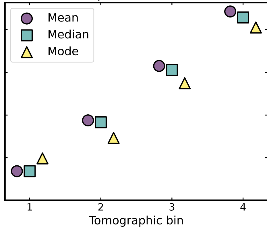
Equidistant bins
