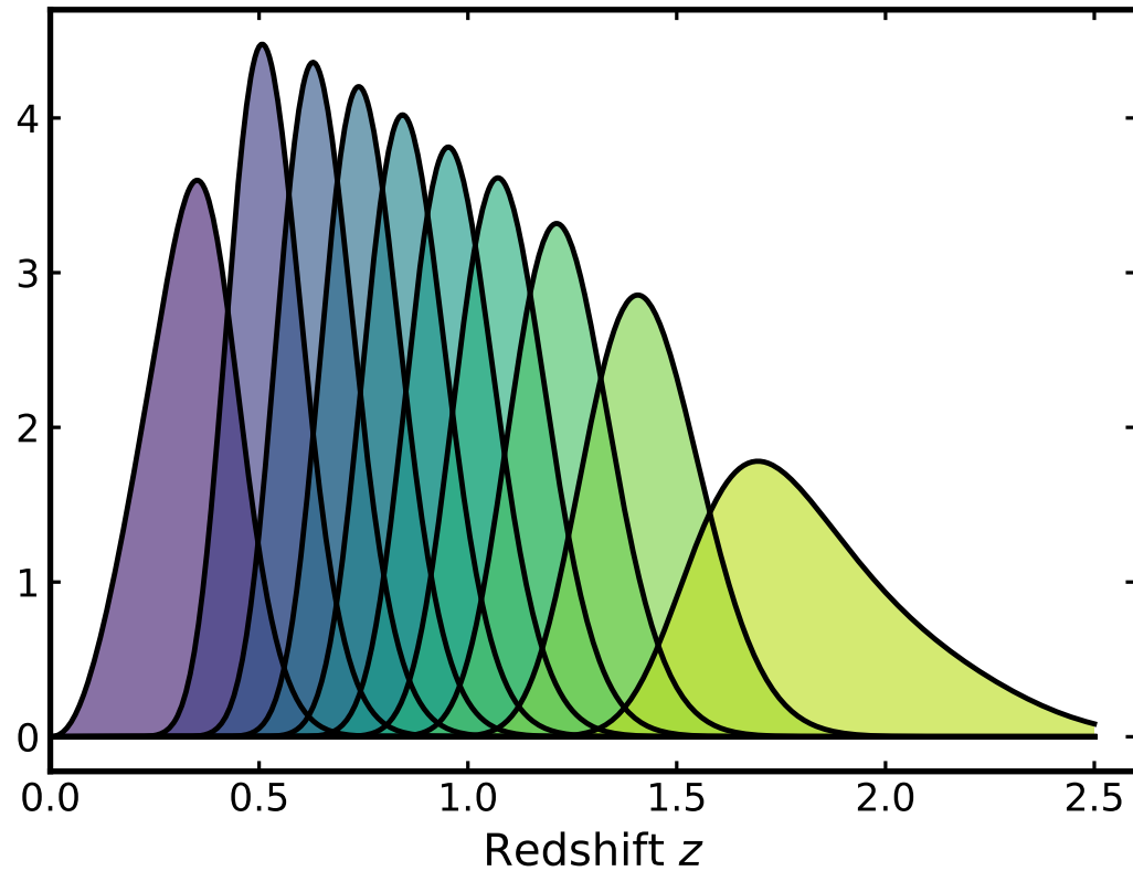
Euclid source bins
