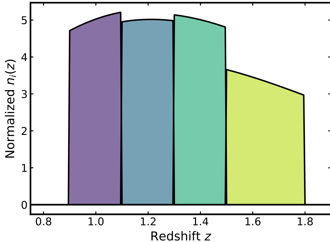
Euclid lens bins
