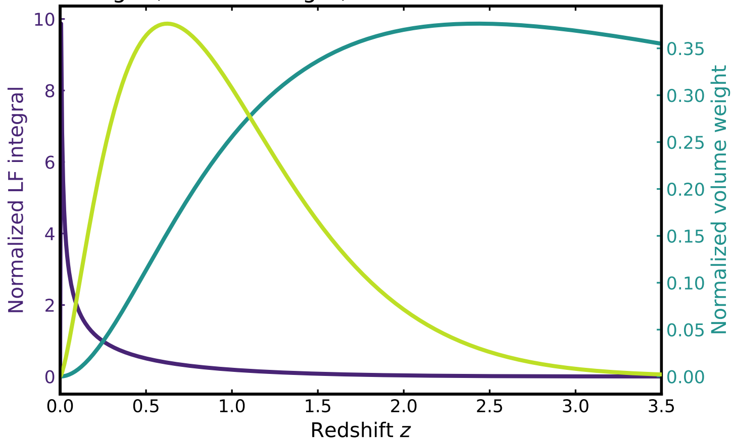
LF integral, volume weight, and final redshift distribution
