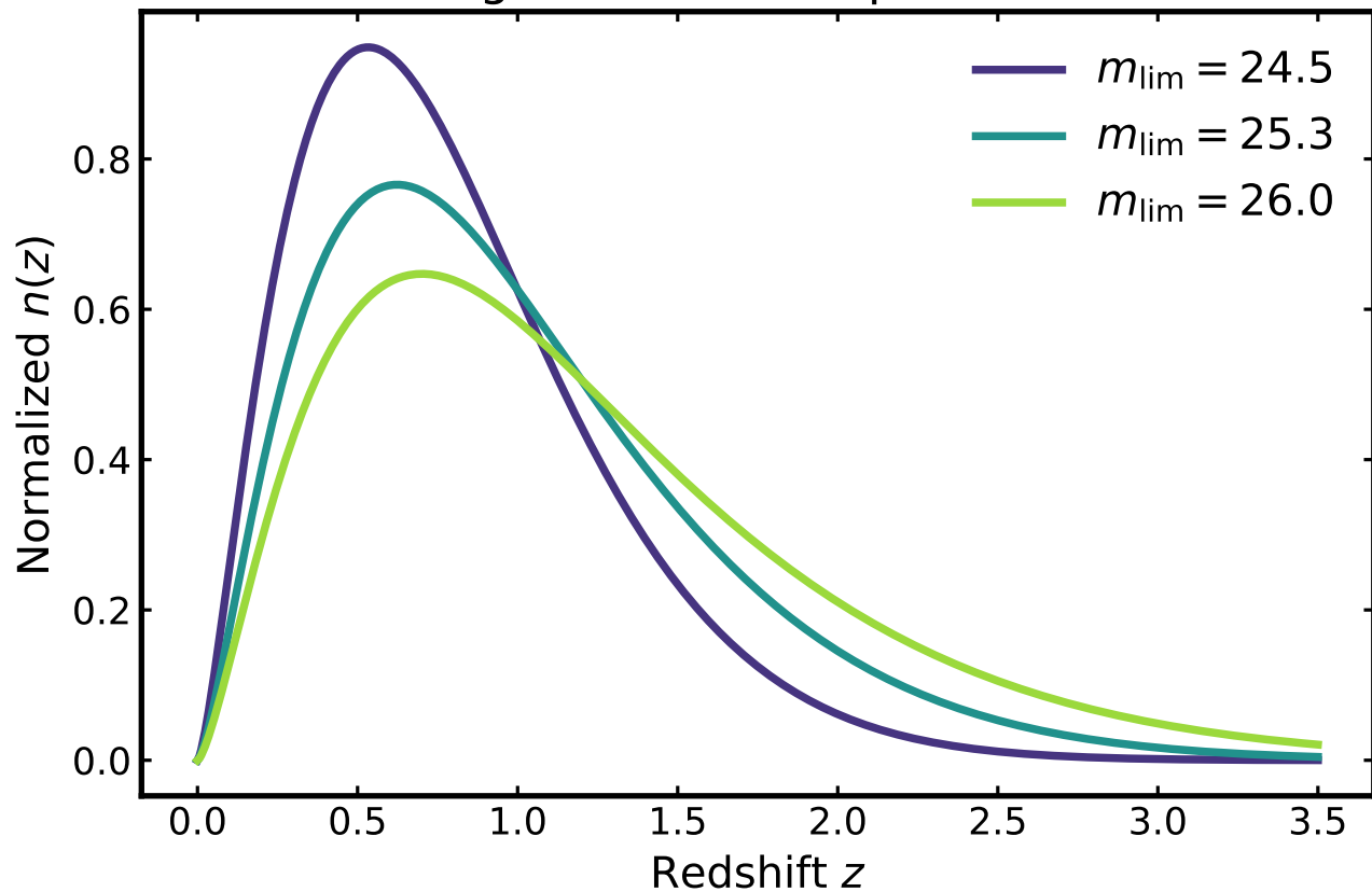
Magnitude-limit dependence
