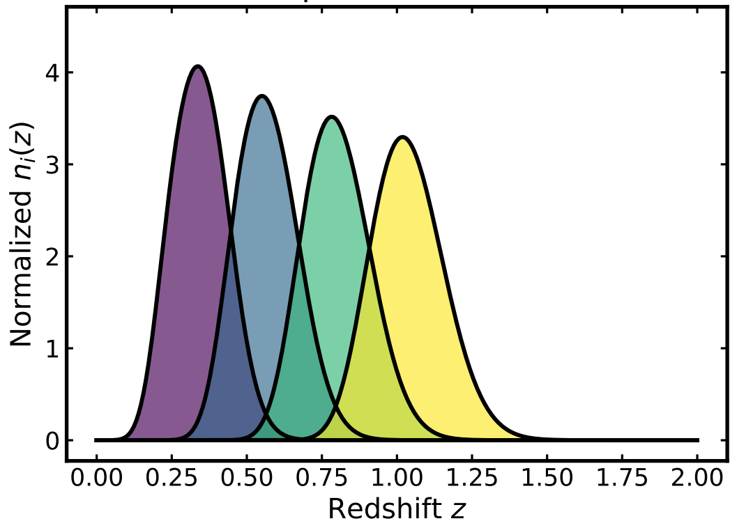
Equidistant bins
